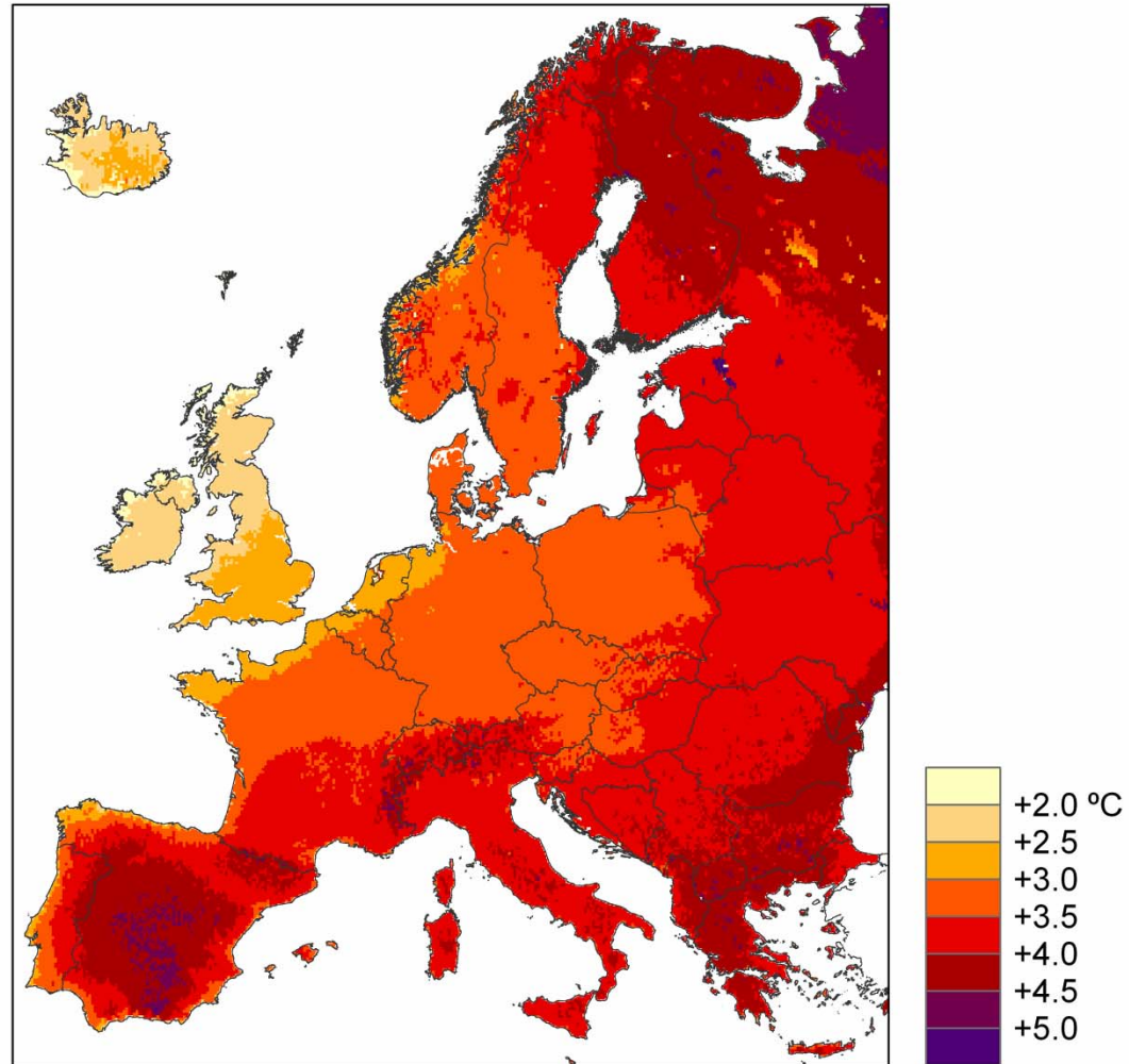
Temperature: change in mean annual temperature
