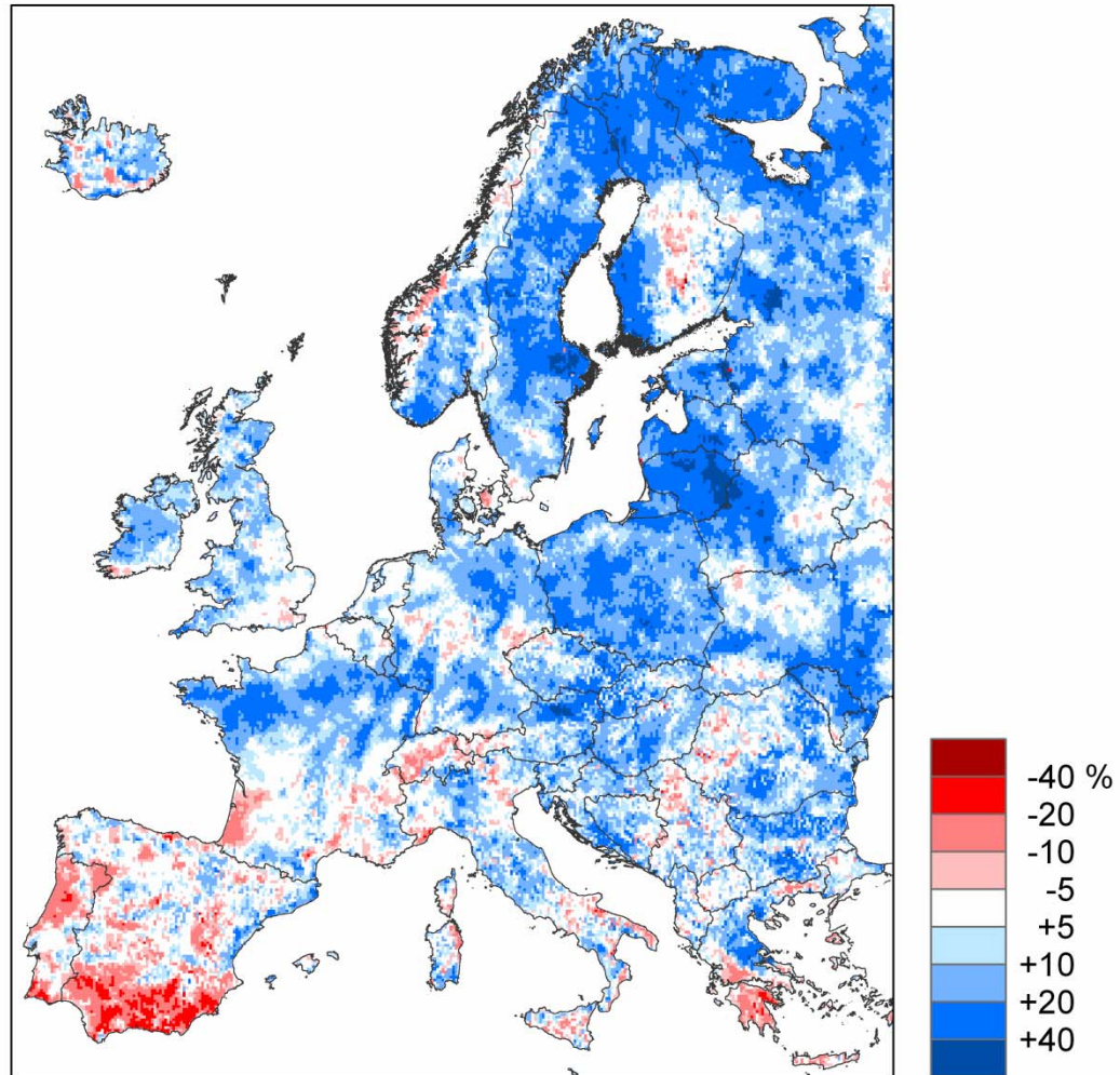
Precipitation: change in annual maximum 5-day amount
